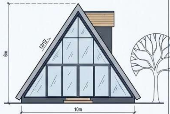
3 BACK (PRIVATE/TREE) ELEVATION Scale 1:100
