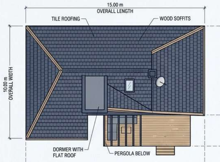
ROOF (ROOF PLAN) Scale 1:100
