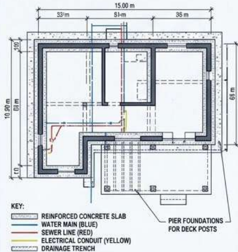
5 SUBSURFACE (FOUNDATIONS & UTILITIES) PLAN Scale 1:100
